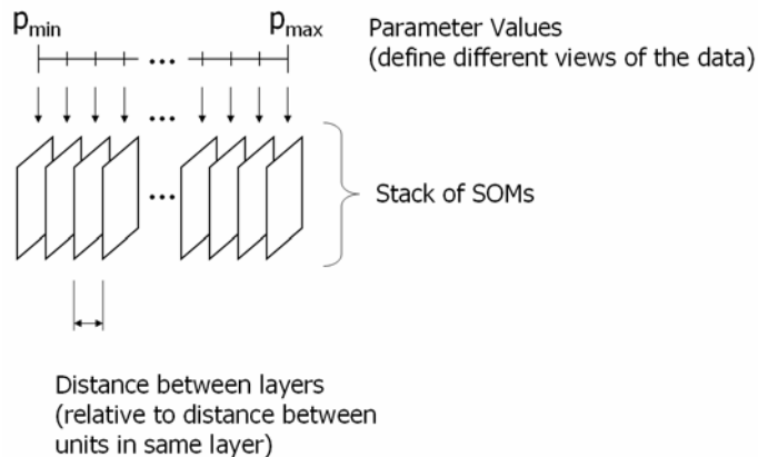
Figure 4 This figure shows the basic architecture of Aligned SOMs.
