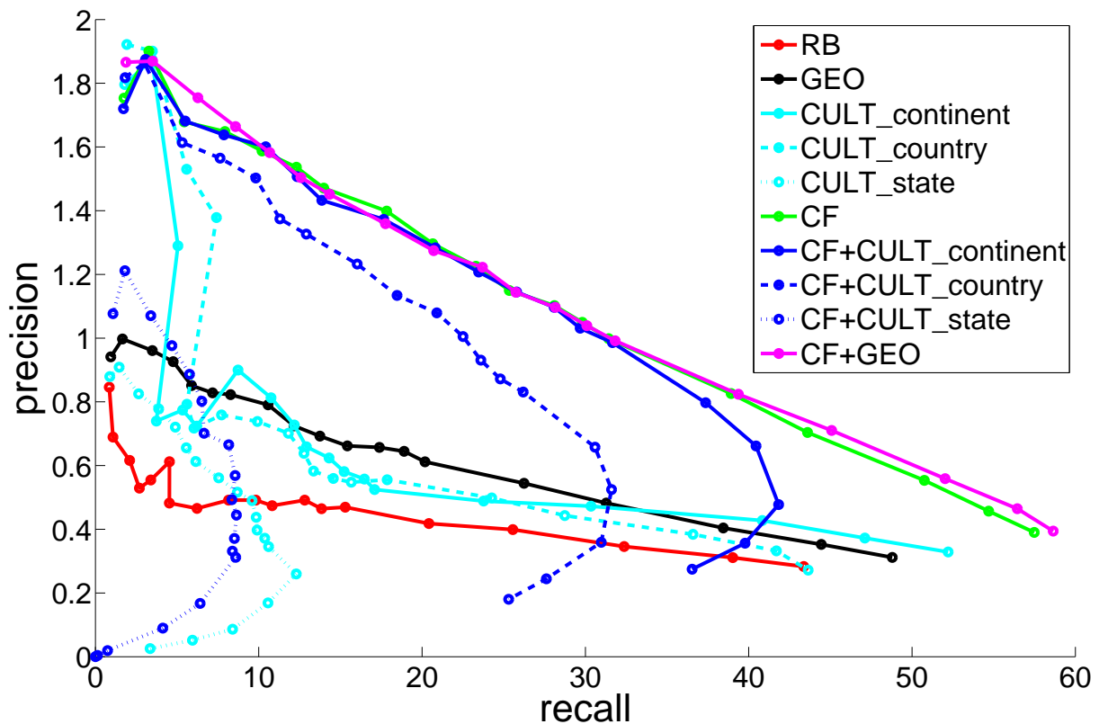
Figure 1: Precision/recall plot.
